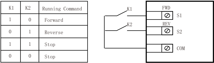
Two-wire 1 sequence wiring diagram
