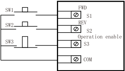
Three-wire 1 sequence wiring diagram
